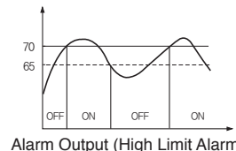
Alarm Output (High Limit Alarm) [AtS=70, AdF=5, AdL=0, SAo=0]
