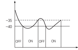
Alarm Output (Low Limit Alarm) [AtS=-40, AdF=5, AdL=0, SAo=0]
